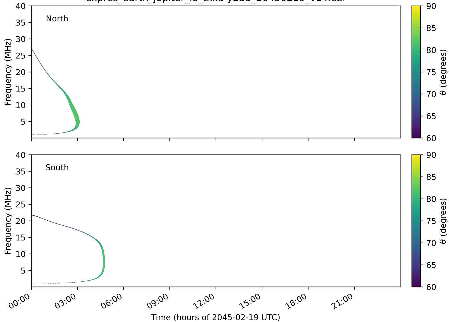
expres_earth_jupiter_io_txka-y235_20450219_v14.cdf
