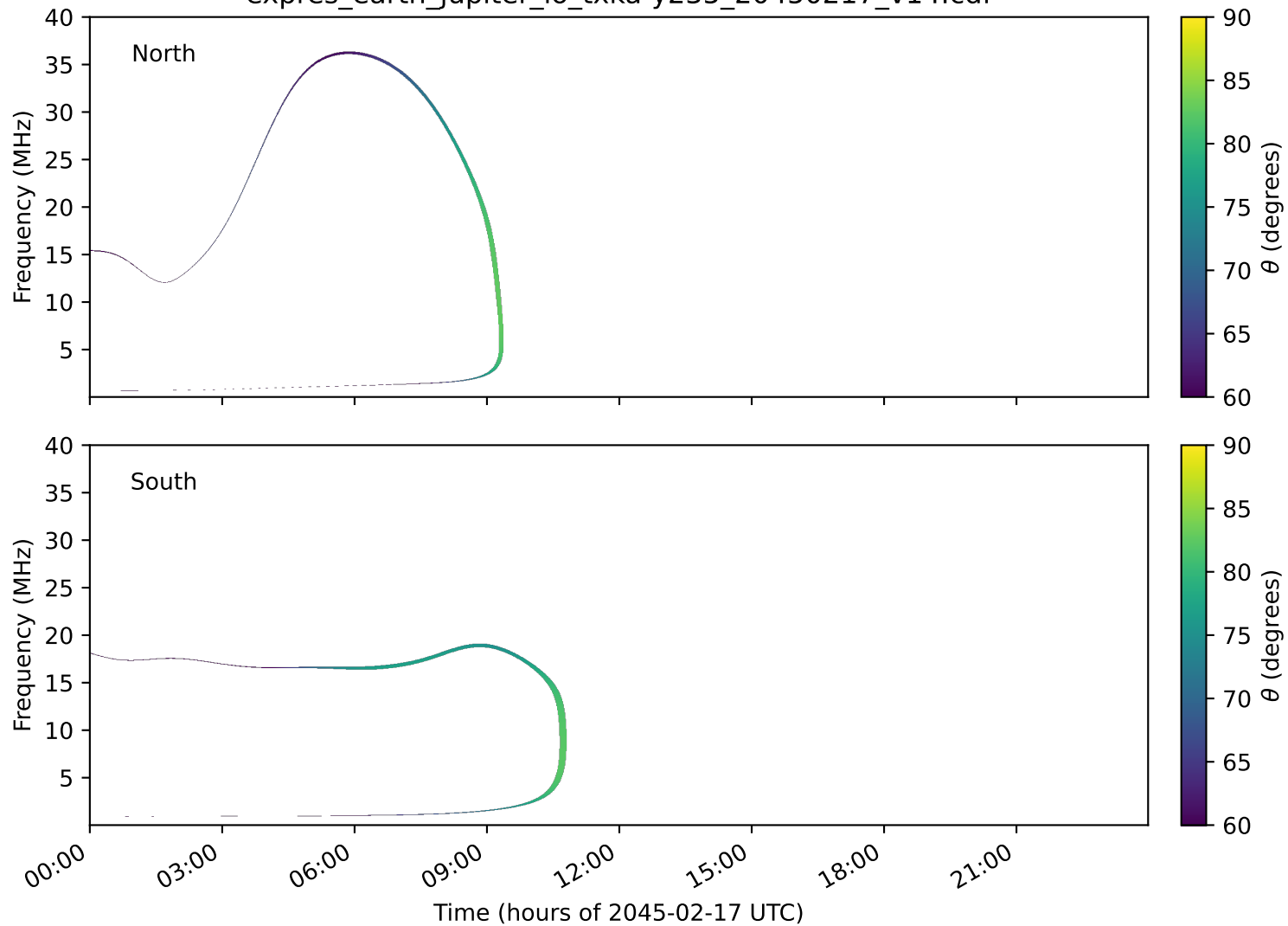
expres_earth_jupiter_io_txka-y235_20450217_v14.cdf
