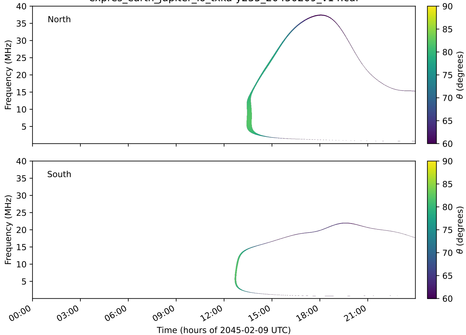
expres_earth_jupiter_io_txka-y235_20450209_v14.cdf
