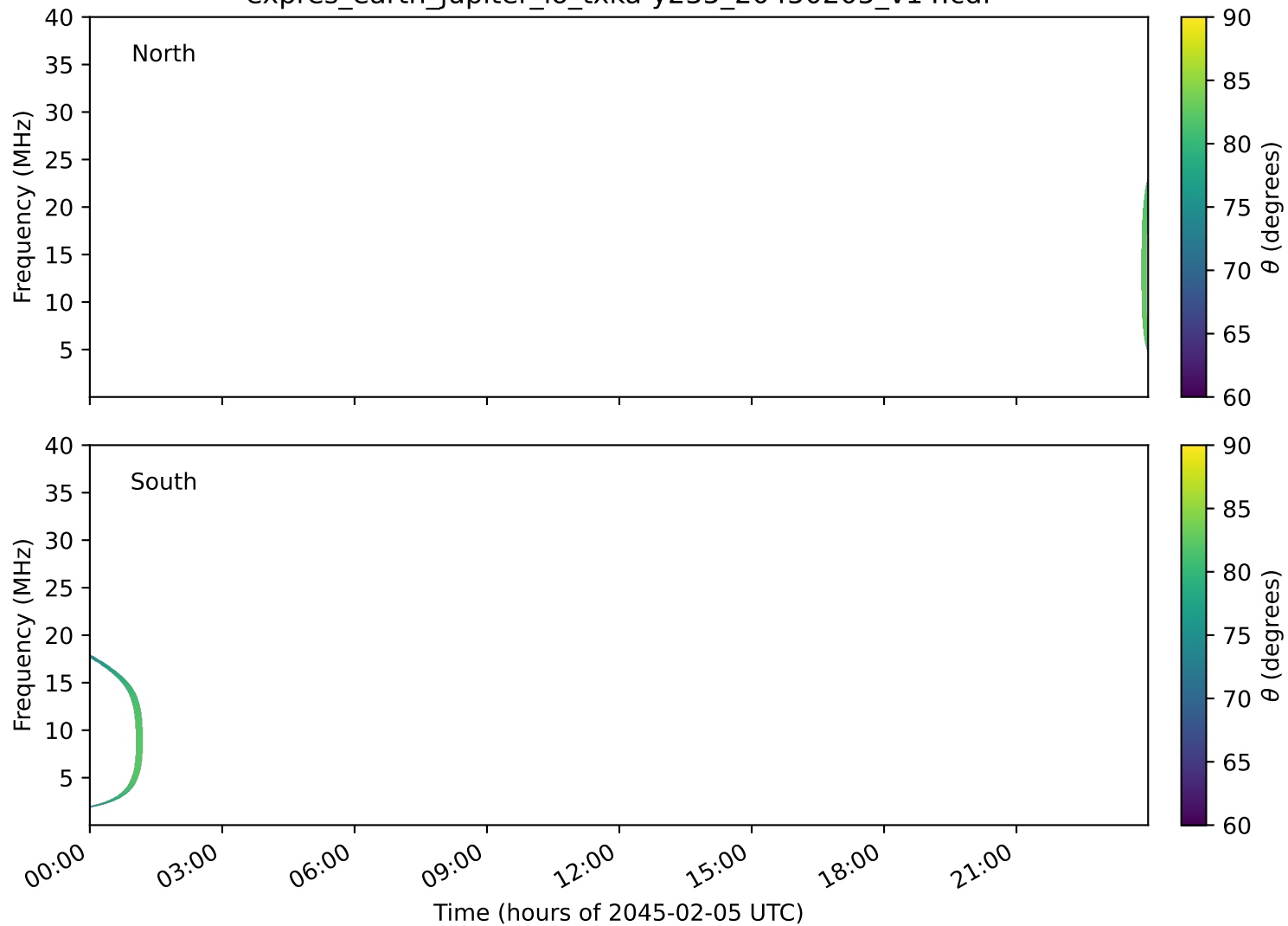
expres_earth_jupiter_io_txka-y235_20450205_v14.cdf
