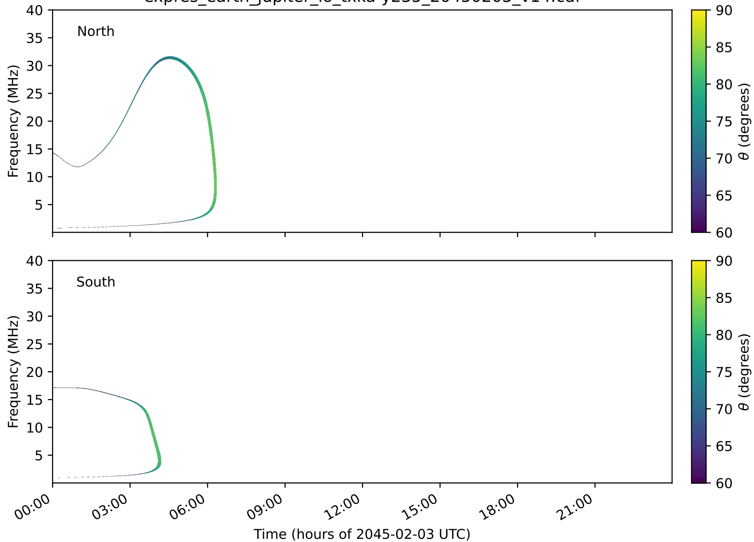
expres_earth_jupiter_io_txka-y235_20450203_v14.cdf
