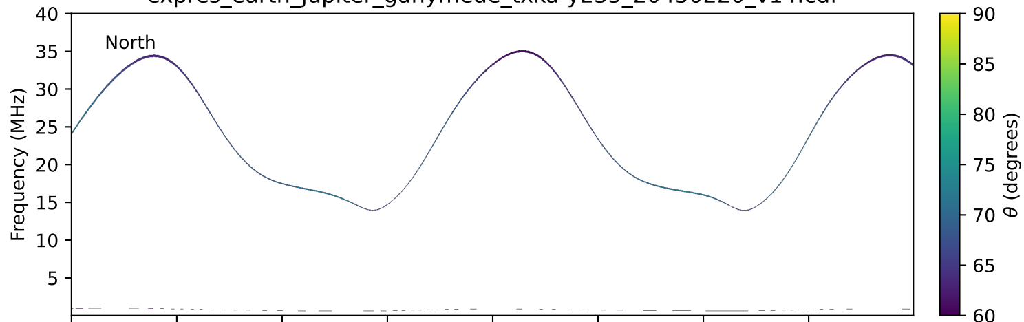
expres_earth_jupiter_ganymede_txka-y235_20450220_v14.cdf
