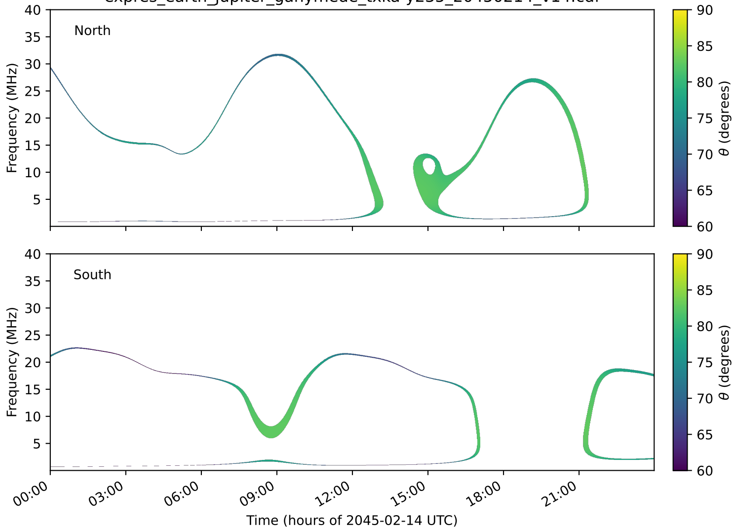
expres_earth_jupiter_ganymede_txka-y235_20450214_v14.cdf
