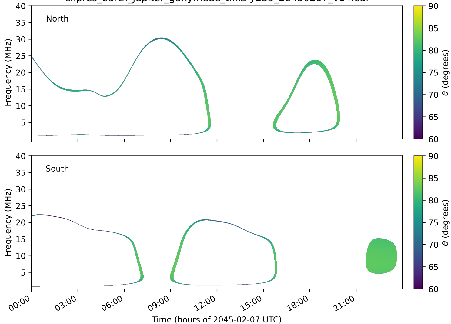
expres_earth_jupiter_ganymede_txka-y235_20450207_v14.cdf
