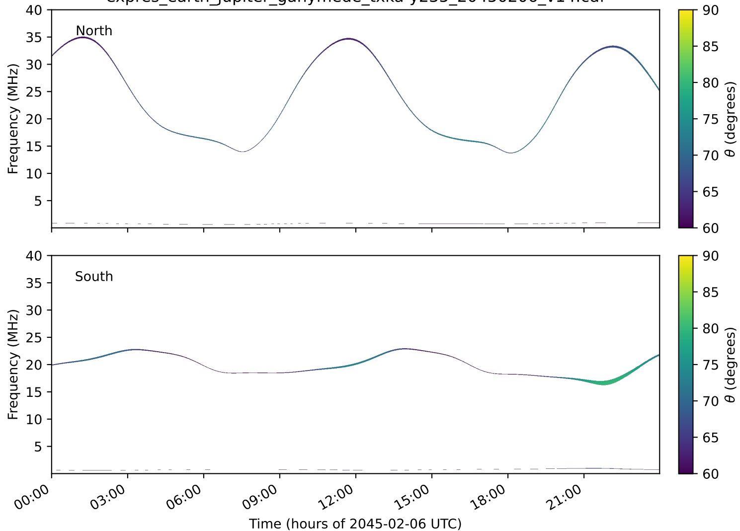
expres_earth_jupiter_ganymede_txka-y235_20450206_v14.cdf
