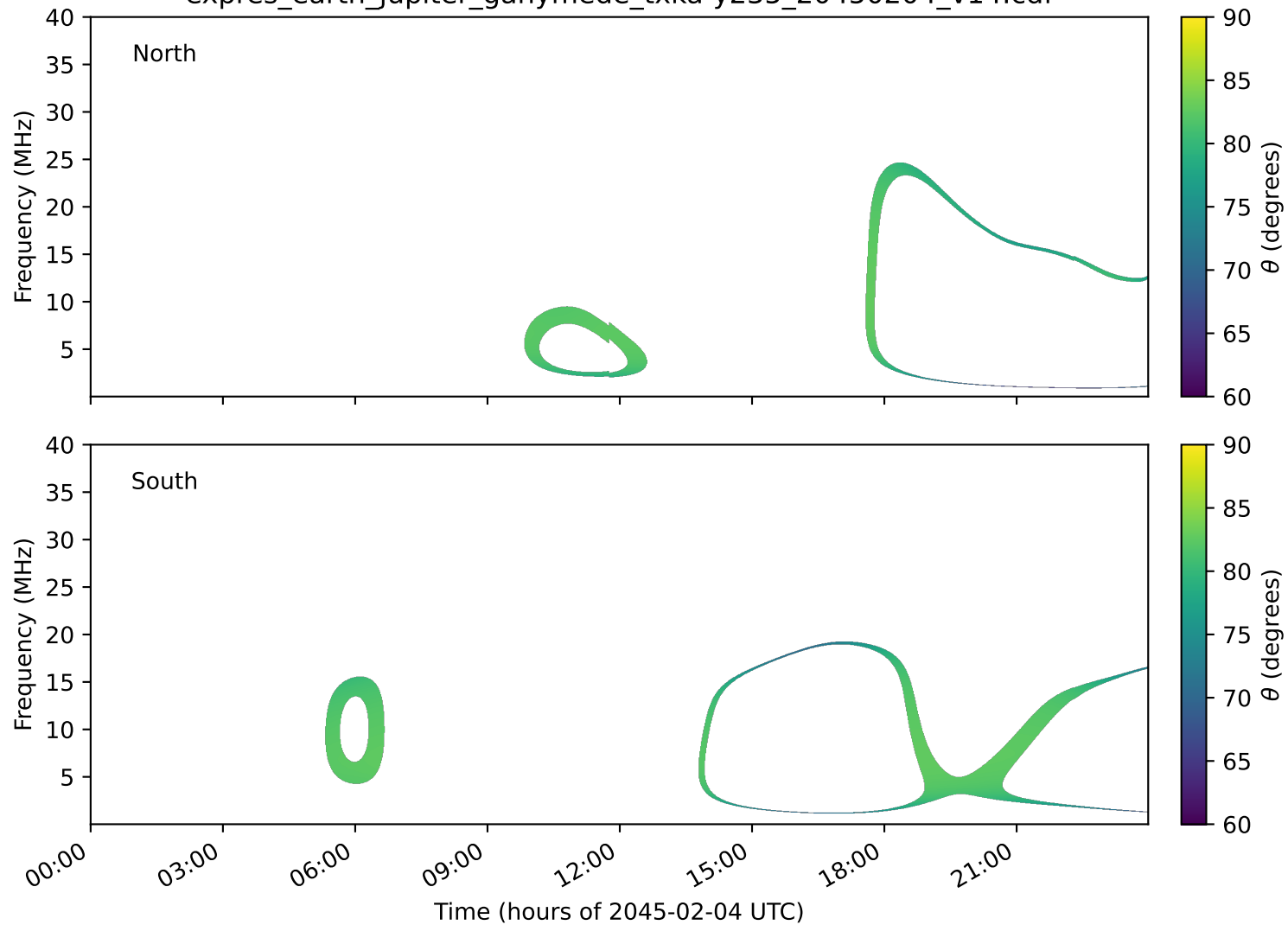
expres_earth_jupiter_ganymede_txka-y235_20450204_v14.cdf
