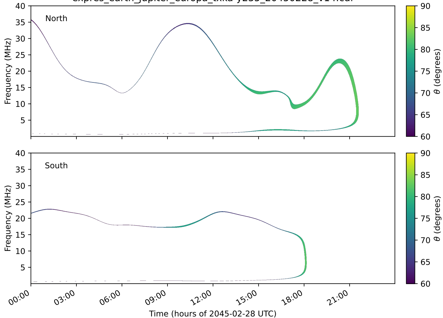
expres_earth_jupiter_europa_txka-y235_20450228_v14.cdf
