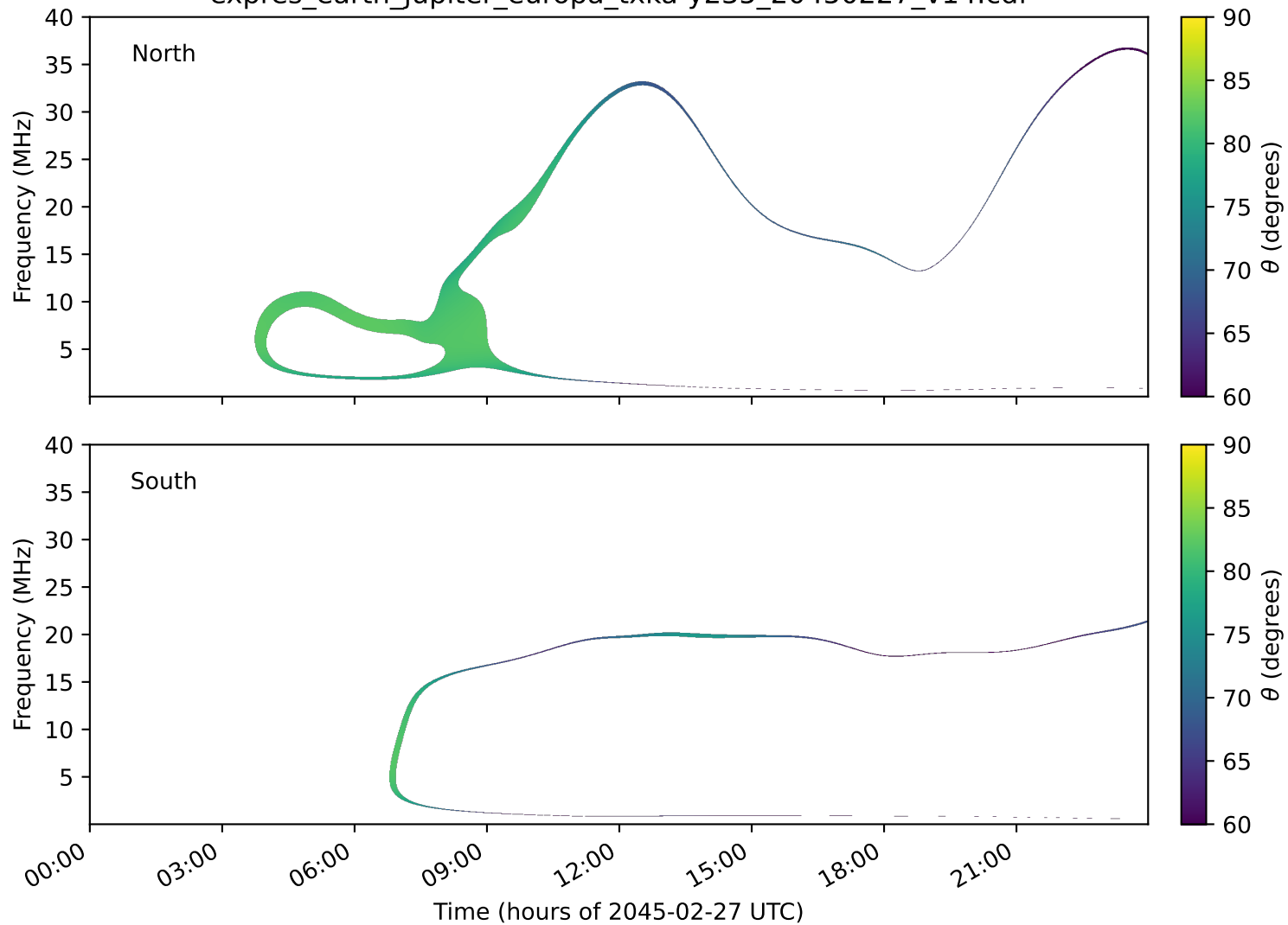
expres_earth_jupiter_europa_txka-y235_20450227_v14.cdf
