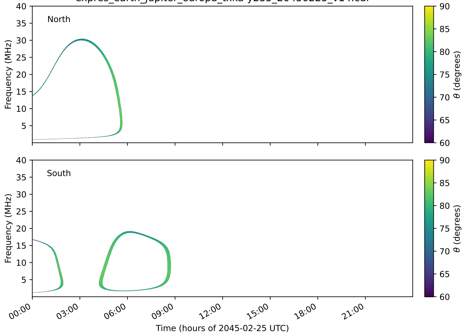
expres_earth_jupiter_europa_txka-y235_20450225_v14.cdf
