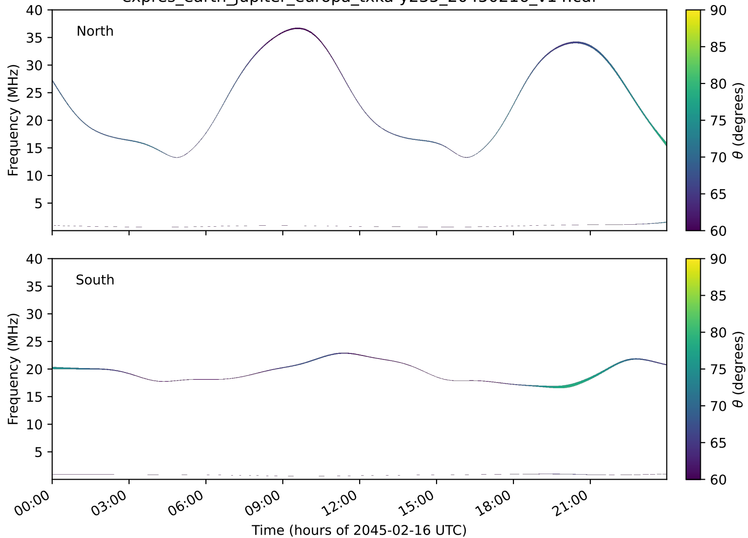
expres_earth_jupiter_europa_txka-y235_20450216_v14.cdf
