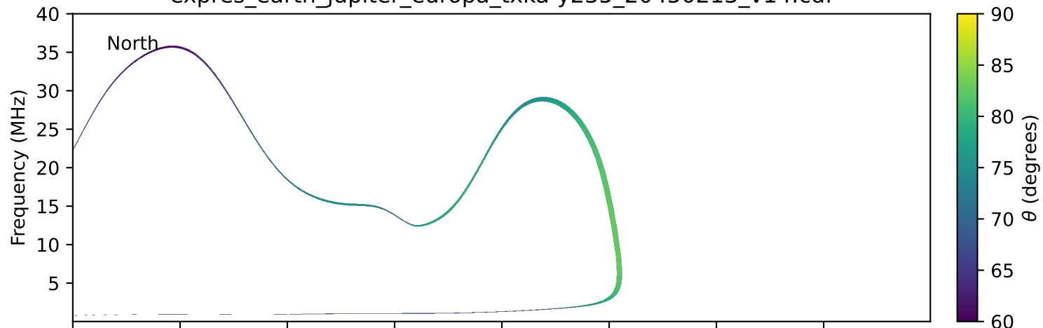
expres_earth_jupiter_europa_txka-y235_20450213_v14.cdf
