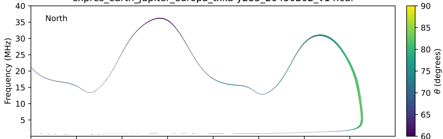
expres_earth_jupiter_europa_txka-y235_20450202_v14.cdf
