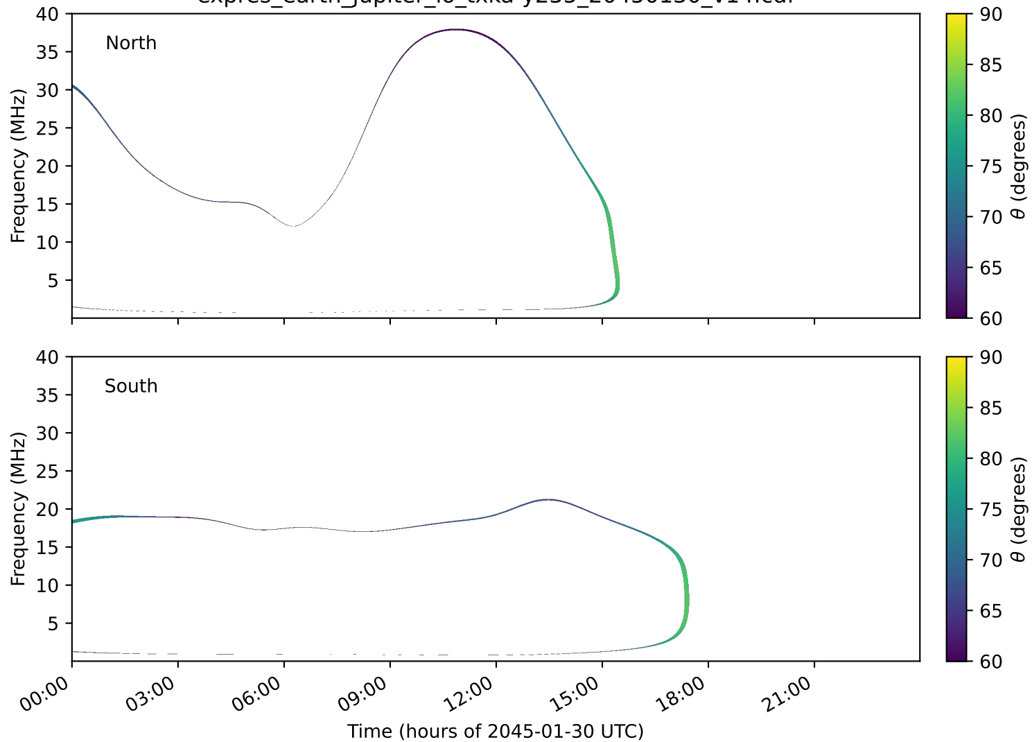
expres_earth_jupiter_io_txka-y235_20450130_v14.cdf
