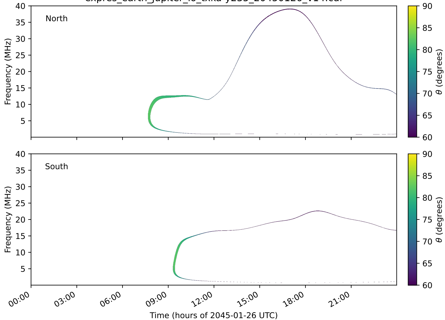
expres_earth_jupiter_io_txka-y235_20450126_v14.cdf
