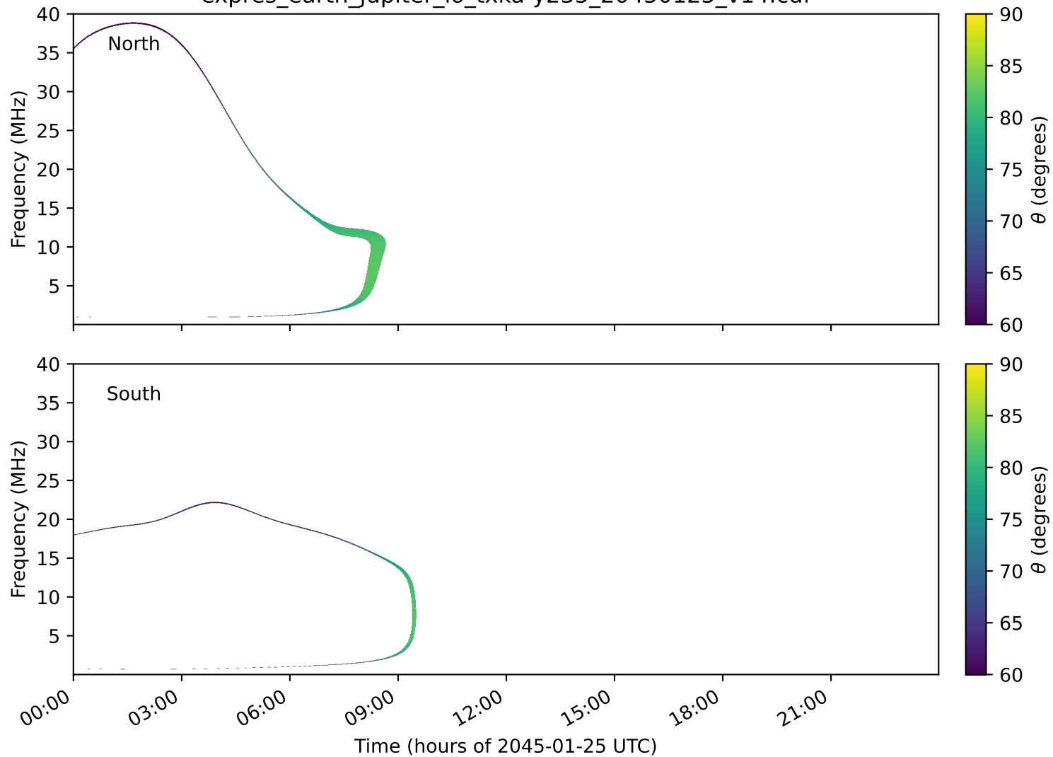
expres_earth_jupiter_io_txka-y235_20450125_v14.cdf
