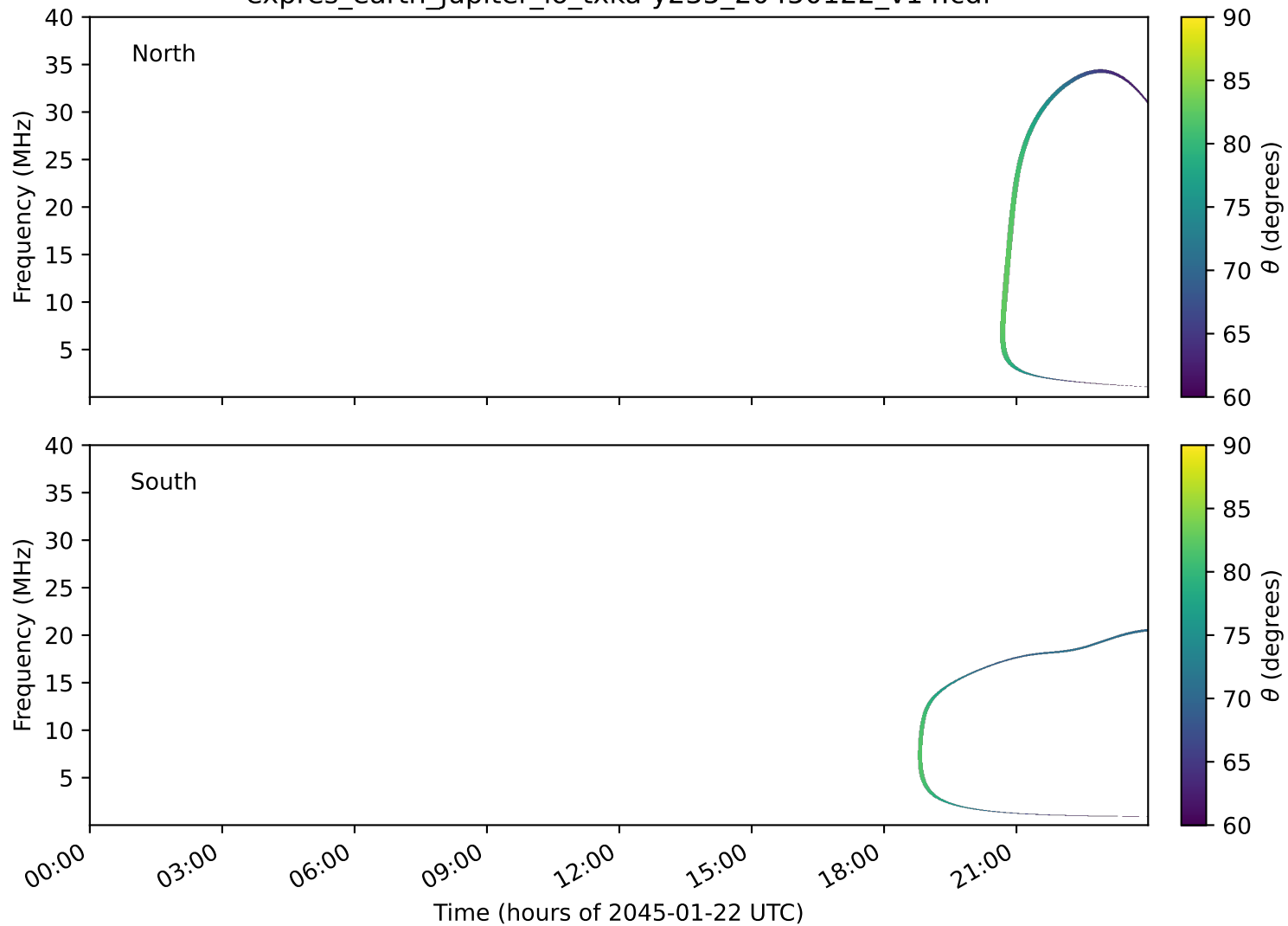
expres_earth_jupiter_io_txka-y235_20450122_v14.cdf
