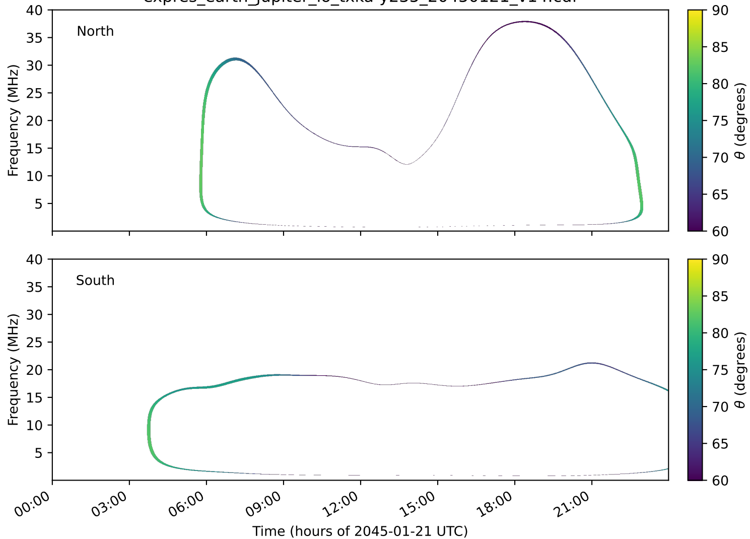
expres_earth_jupiter_io_txka-y235_20450121_v14.cdf
