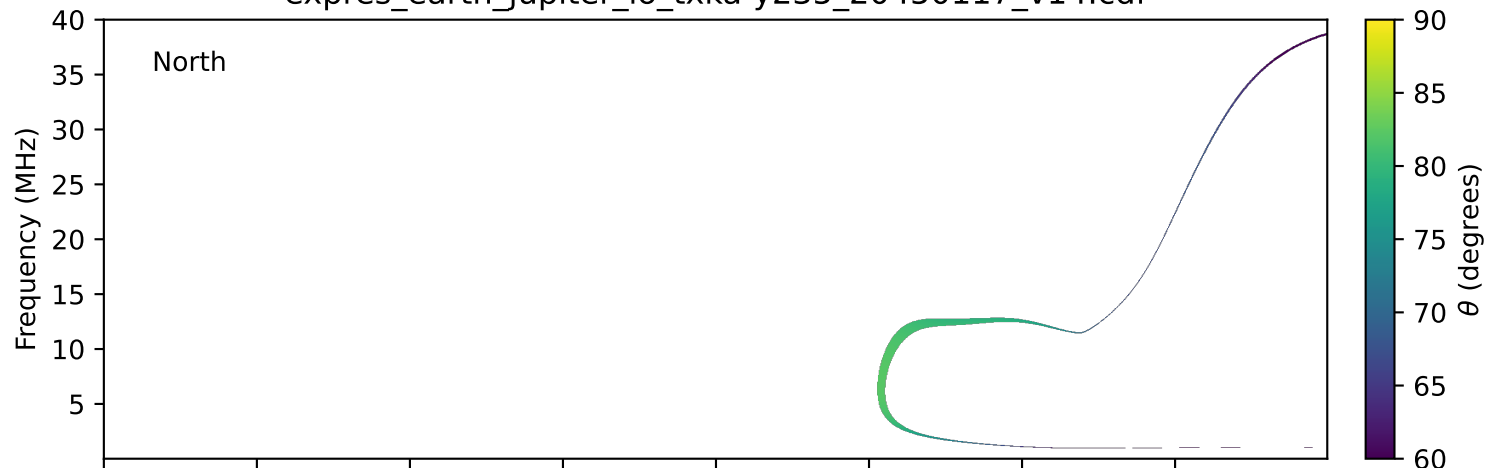
expres_earth_jupiter_io_txka-y235_20450117_v14.cdf
