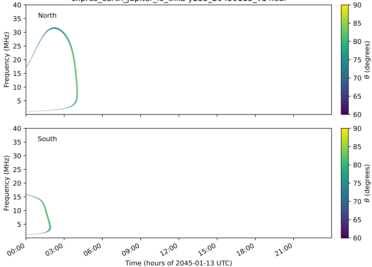
expres_earth_jupiter_io_txka-y235_20450113_v14.cdf
