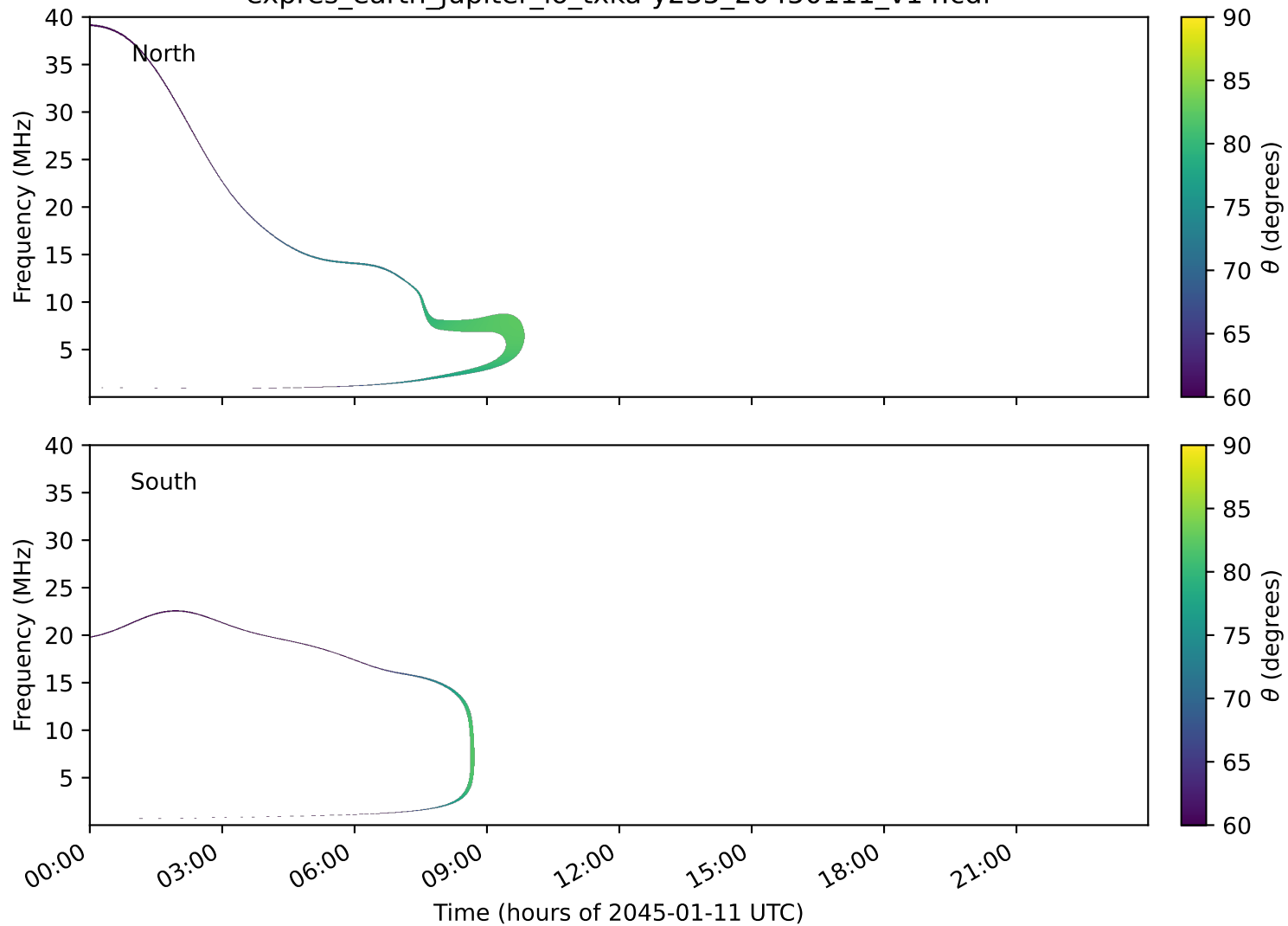
expres_earth_jupiter_io_txka-y235_20450111_v14.cdf
