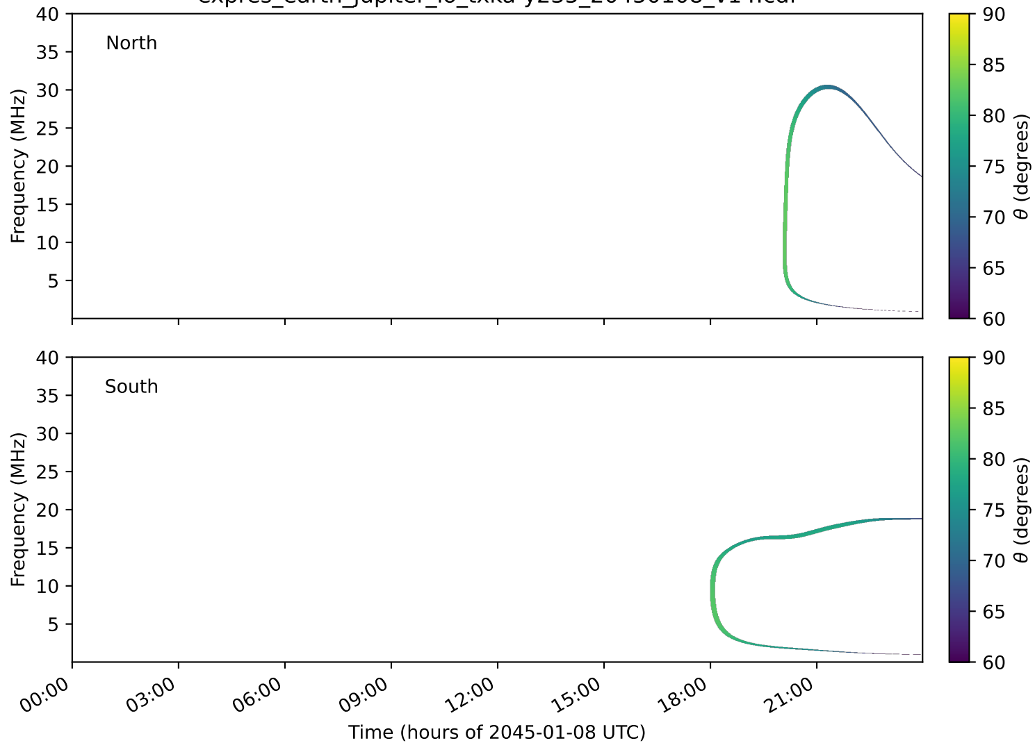
expres_earth_jupiter_io_txka-y235_20450108_v14.cdf
