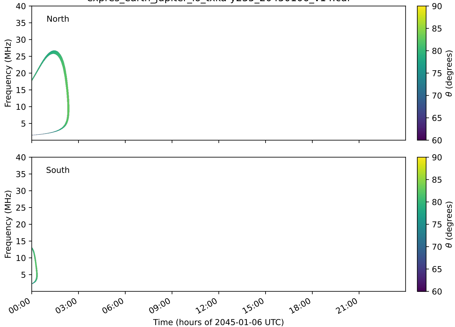
expres_earth_jupiter_io_txka-y235_20450106_v14.cdf
