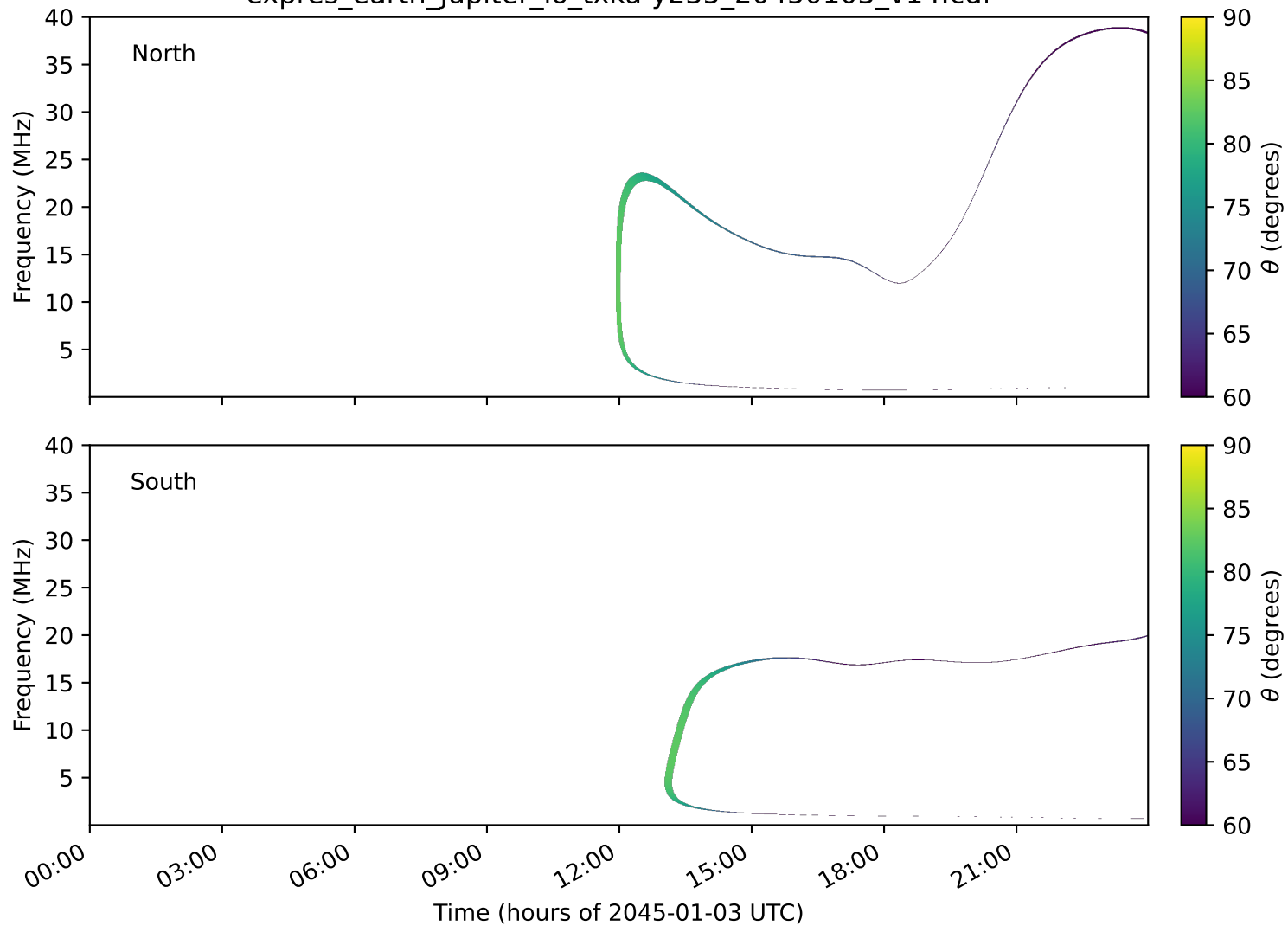
expres_earth_jupiter_io_txka-y235_20450103_v14.cdf
