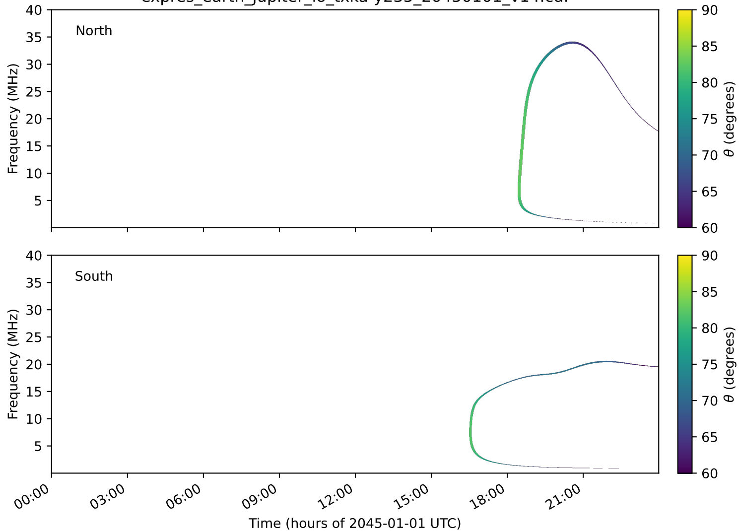
expres_earth_jupiter_io_txka-y235_20450101_v14.cdf
