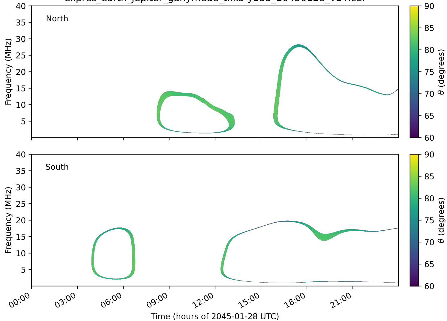
expres_earth_jupiter_ganymede_txka-y235_20450128_v14.cdf
