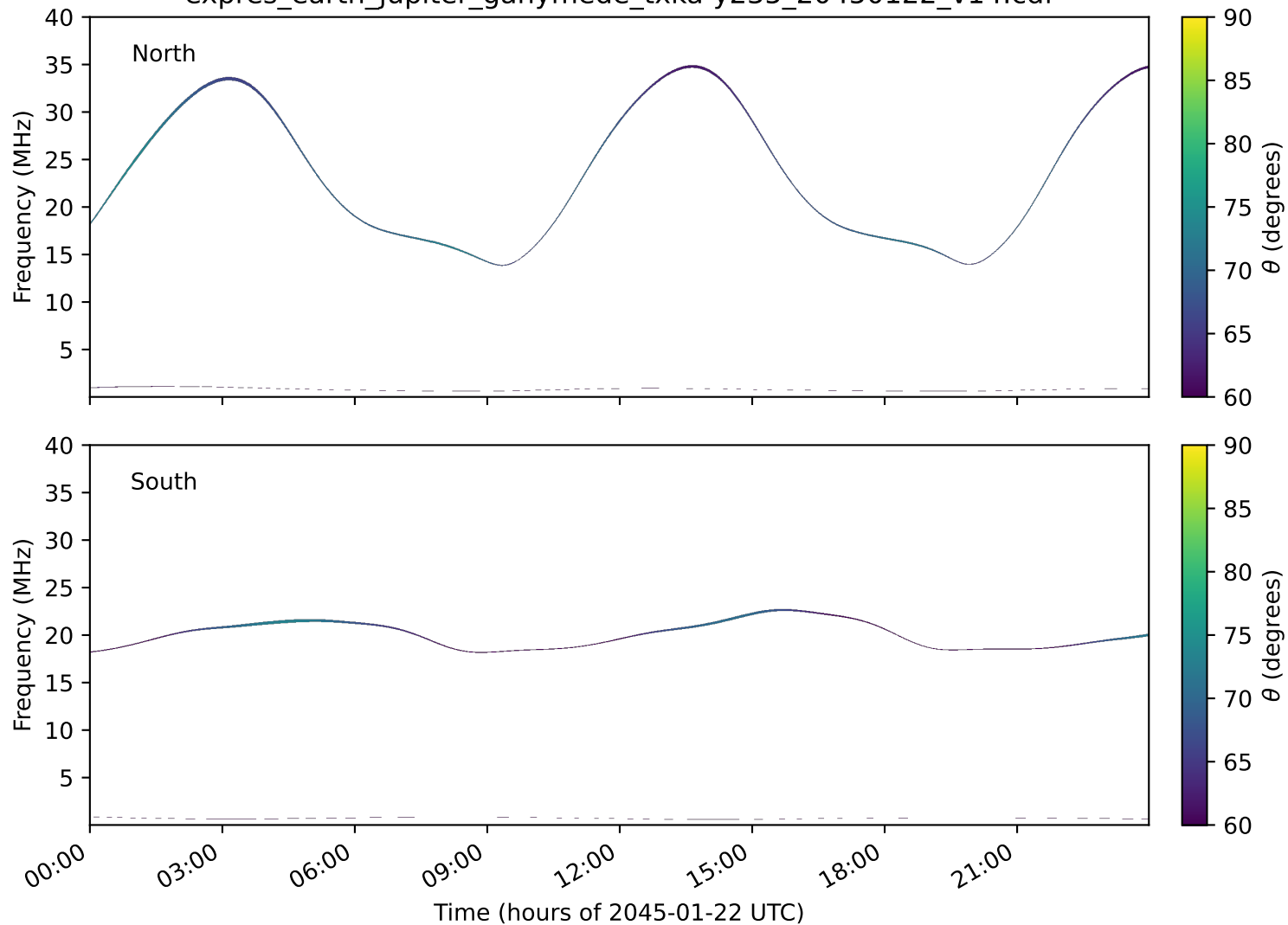
expres_earth_jupiter_ganymede_txka-y235_20450122_v14.cdf
