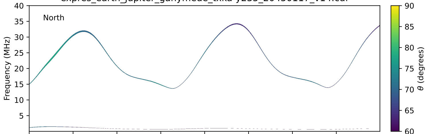
expres_earth_jupiter_ganymede_txka-y235_20450117_v14.cdf
