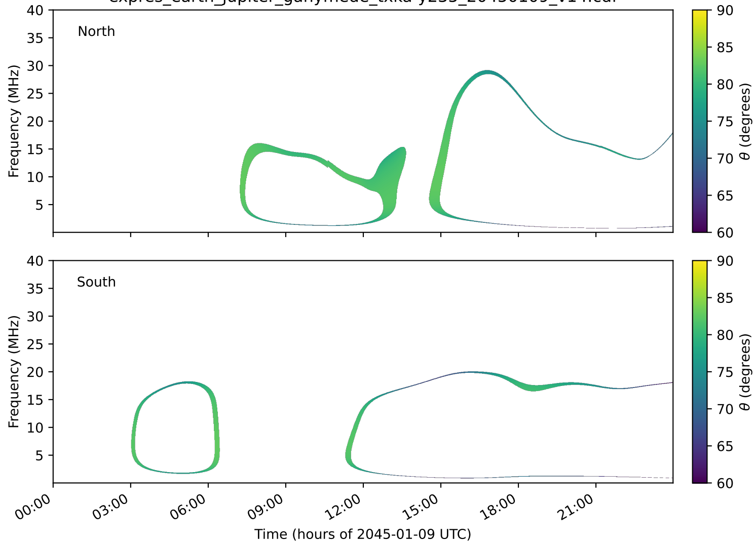
expres_earth_jupiter_ganymede_txka-y235_20450109_v14.cdf
