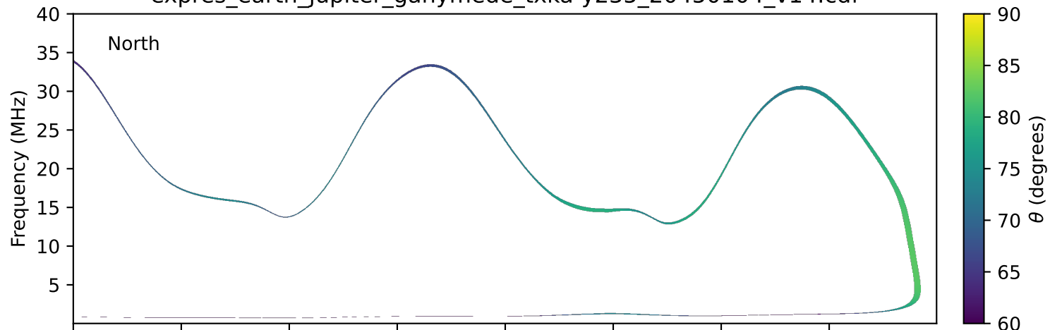
expres_earth_jupiter_ganymede_txka-y235_20450104_v14.cdf
