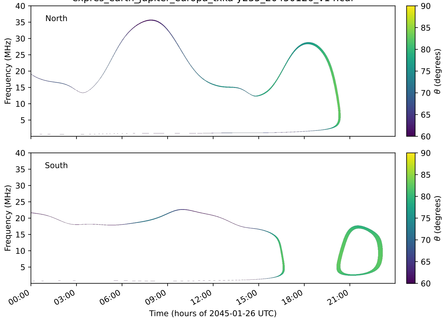
expres_earth_jupiter_europa_txka-y235_20450126_v14.cdf
