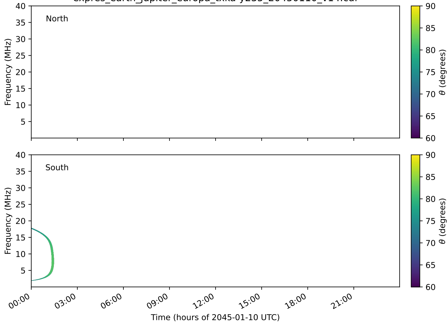
expres_earth_jupiter_europa_txka-y235_20450110_v14.cdf
