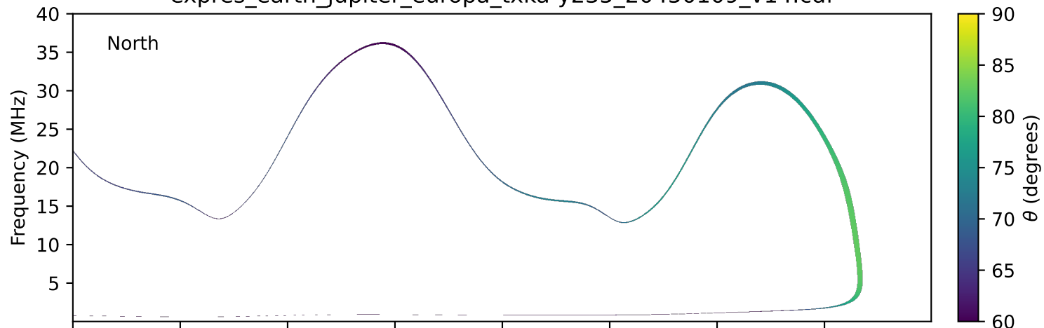
expres_earth_jupiter_europa_txka-y235_20450109_v14.cdf
