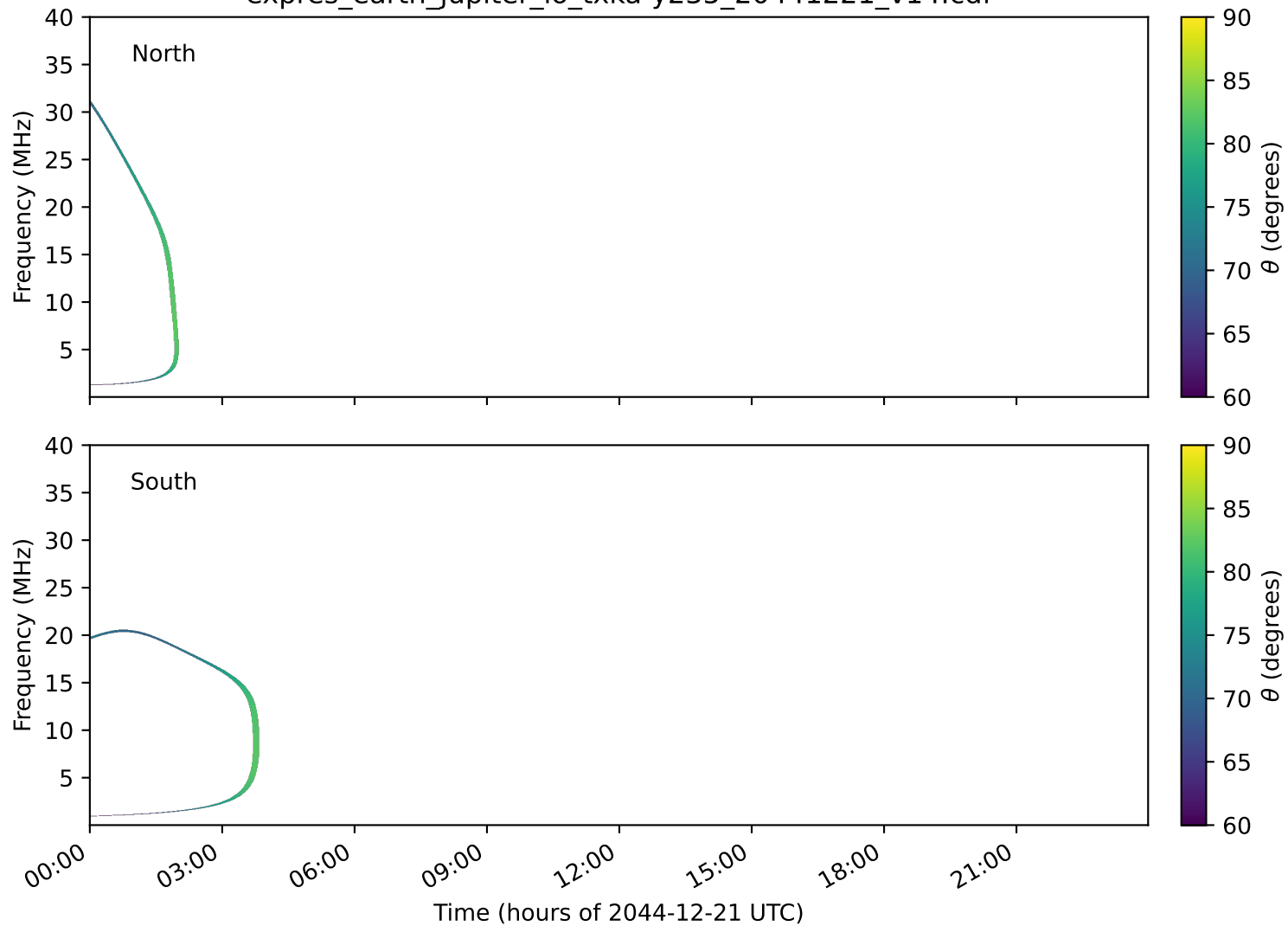
expres_earth_jupiter_io_txka-y235_20441221_v14.cdf
