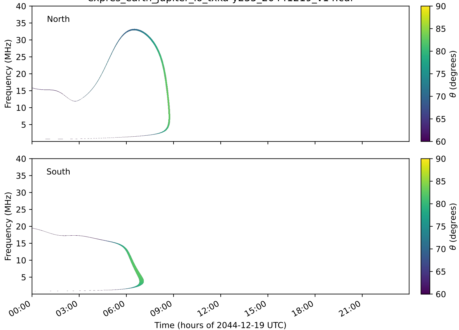
expres_earth_jupiter_io_txka-y235_20441219_v14.cdf
