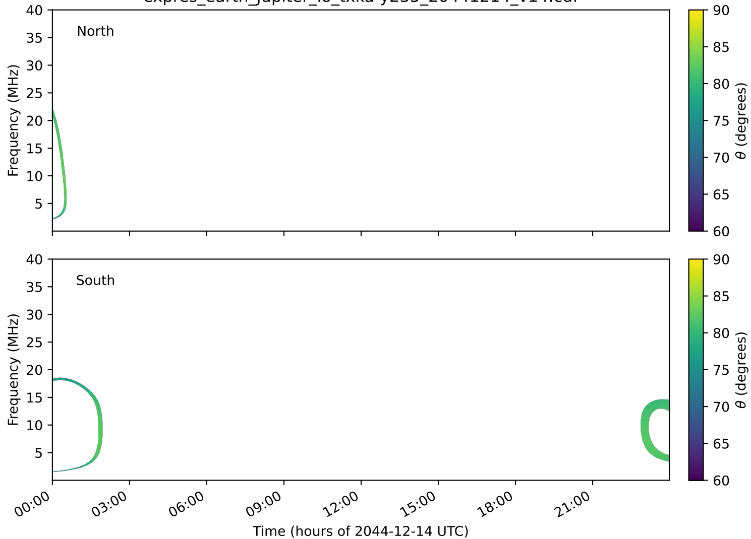
expres_earth_jupiter_io_txka-y235_20441214_v14.cdf
