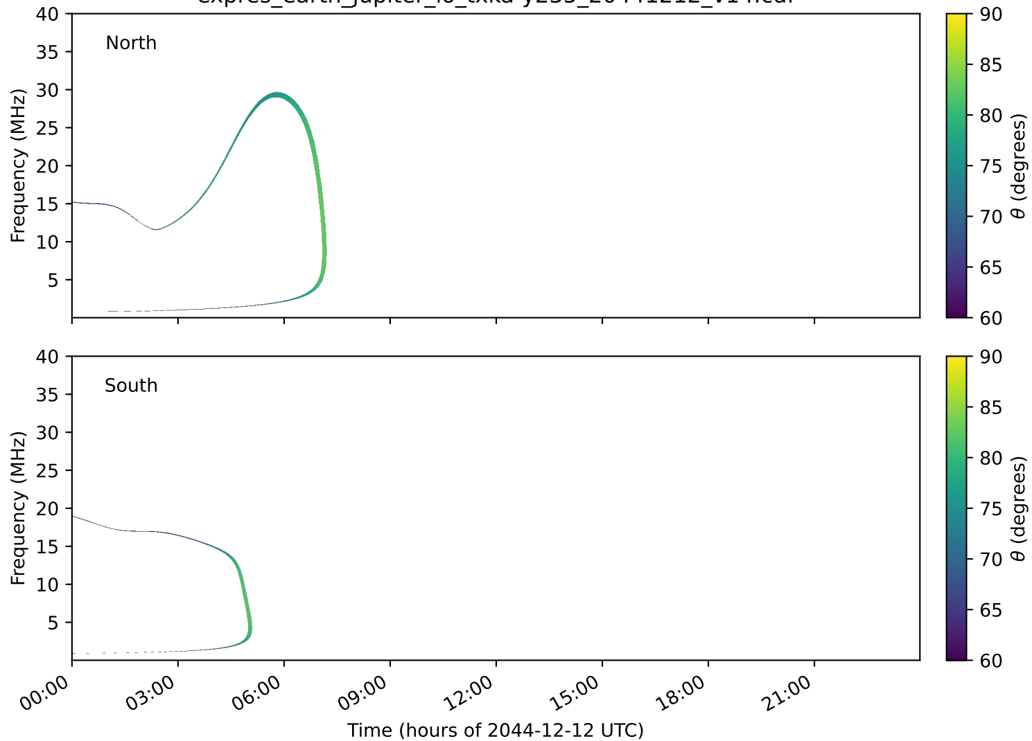
expres_earth_jupiter_io_txka-y235_20441212_v14.cdf
