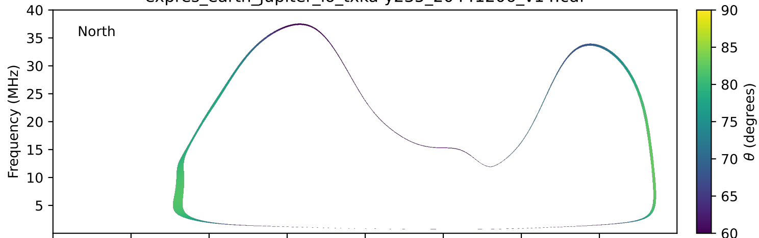
expres_earth_jupiter_io_txka-y235_20441206_v14.cdf
