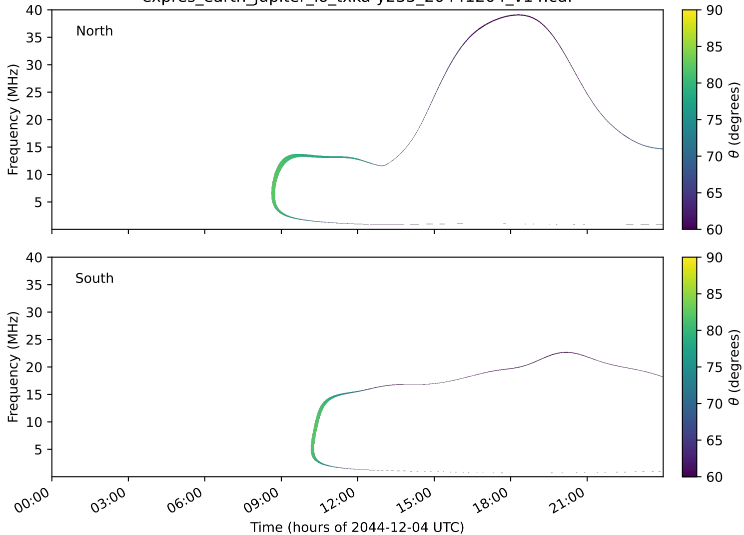
expres_earth_jupiter_io_txka-y235_20441204_v14.cdf
