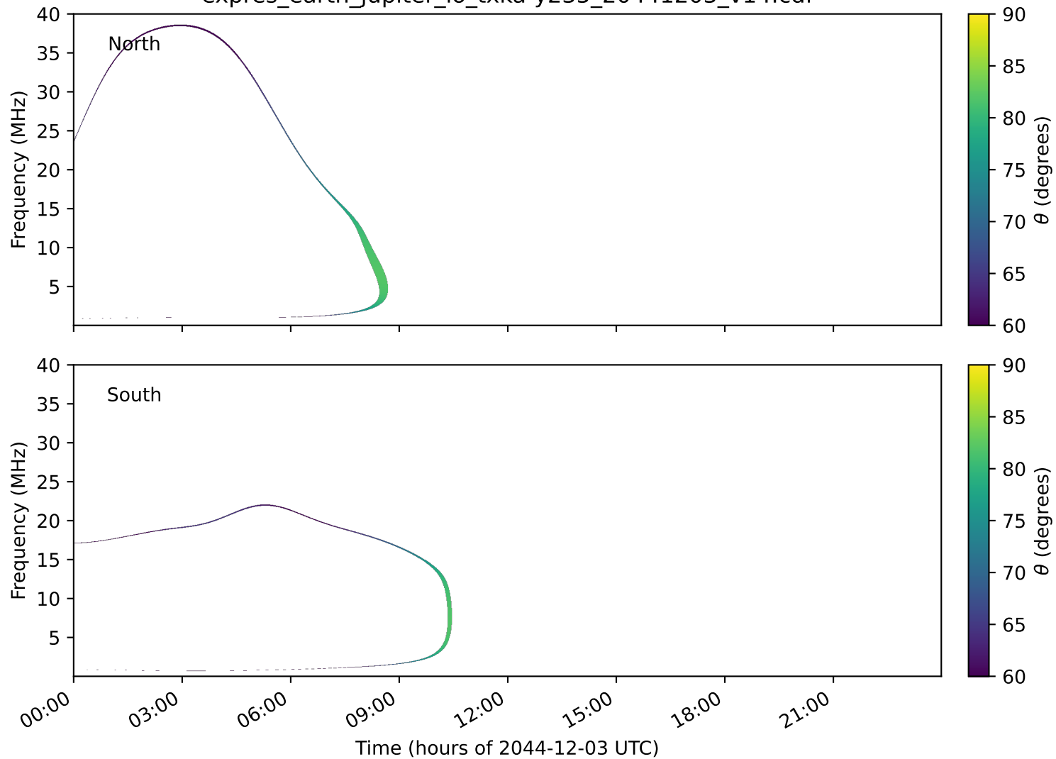
expres_earth_jupiter_io_txka-y235_20441203_v14.cdf
