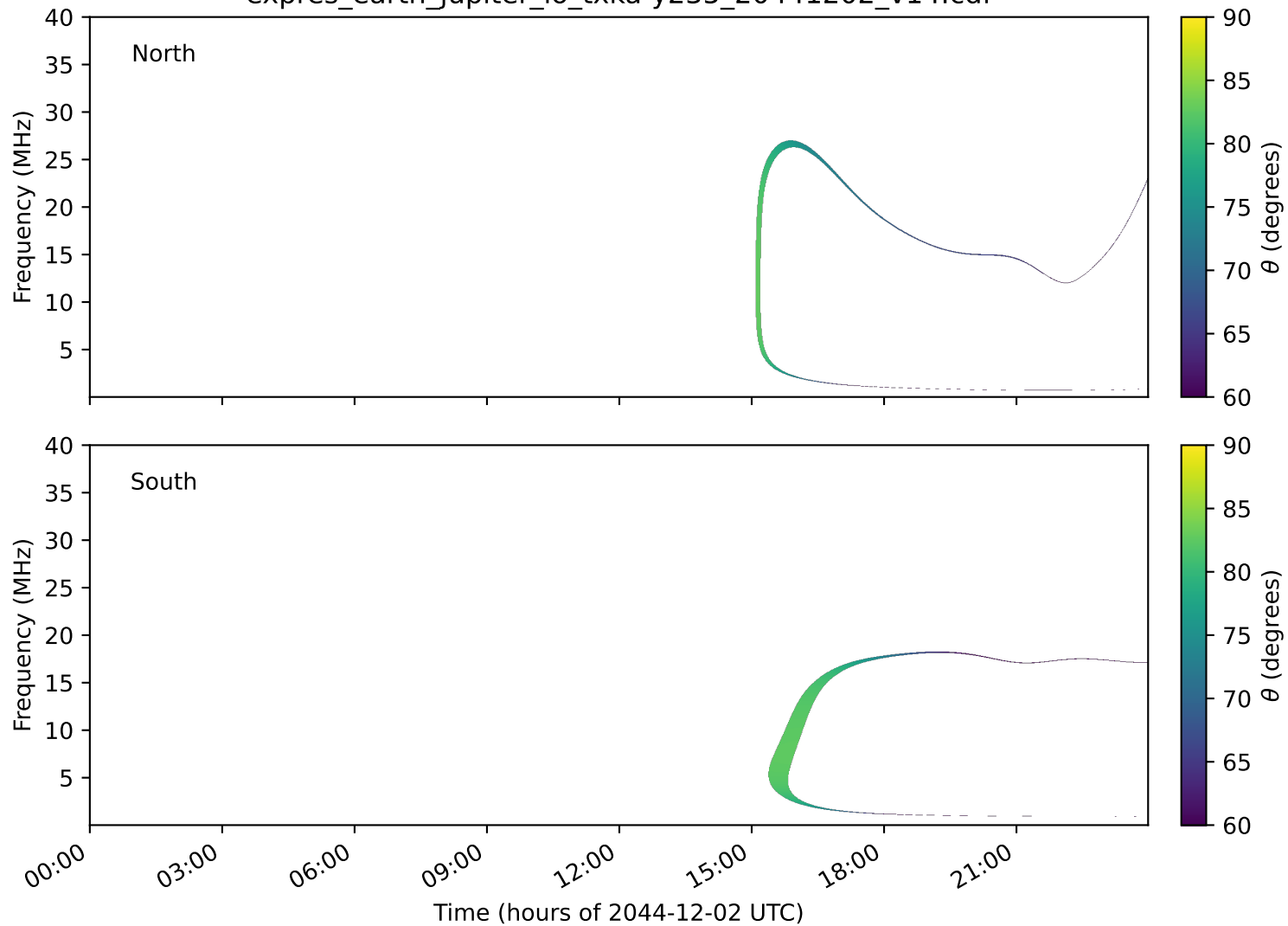
expres_earth_jupiter_io_txka-y235_20441202_v14.cdf
