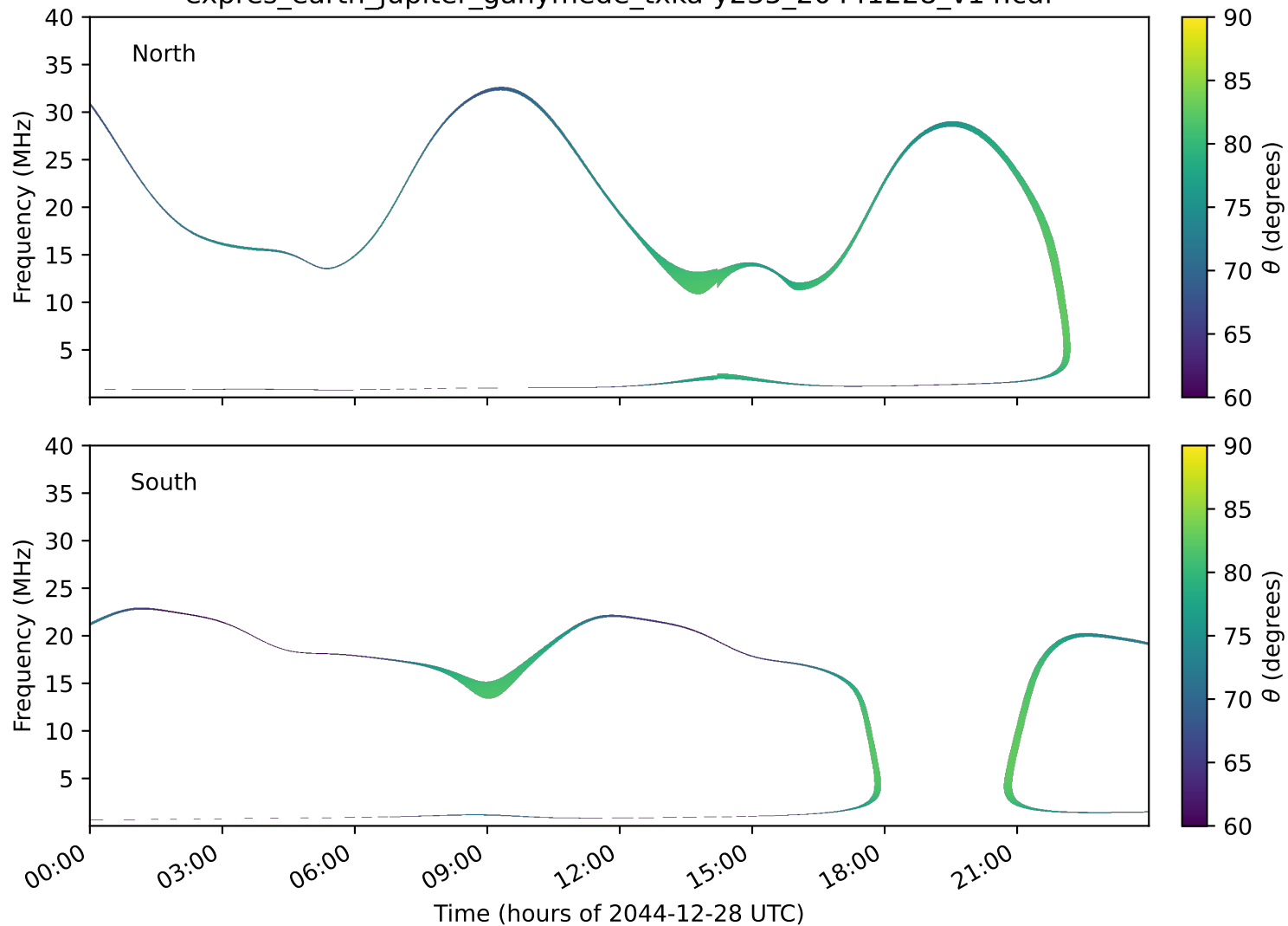
expres_earth_jupiter_ganymede_txka-y235_20441228_v14.cdf
