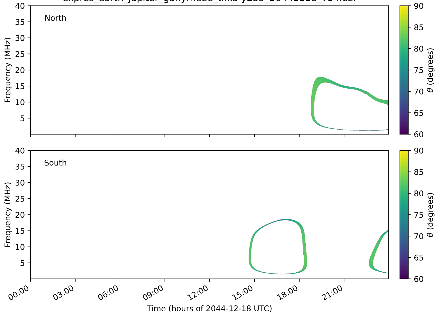
expres_earth_jupiter_ganymede_txka-y235_20441218_v14.cdf
