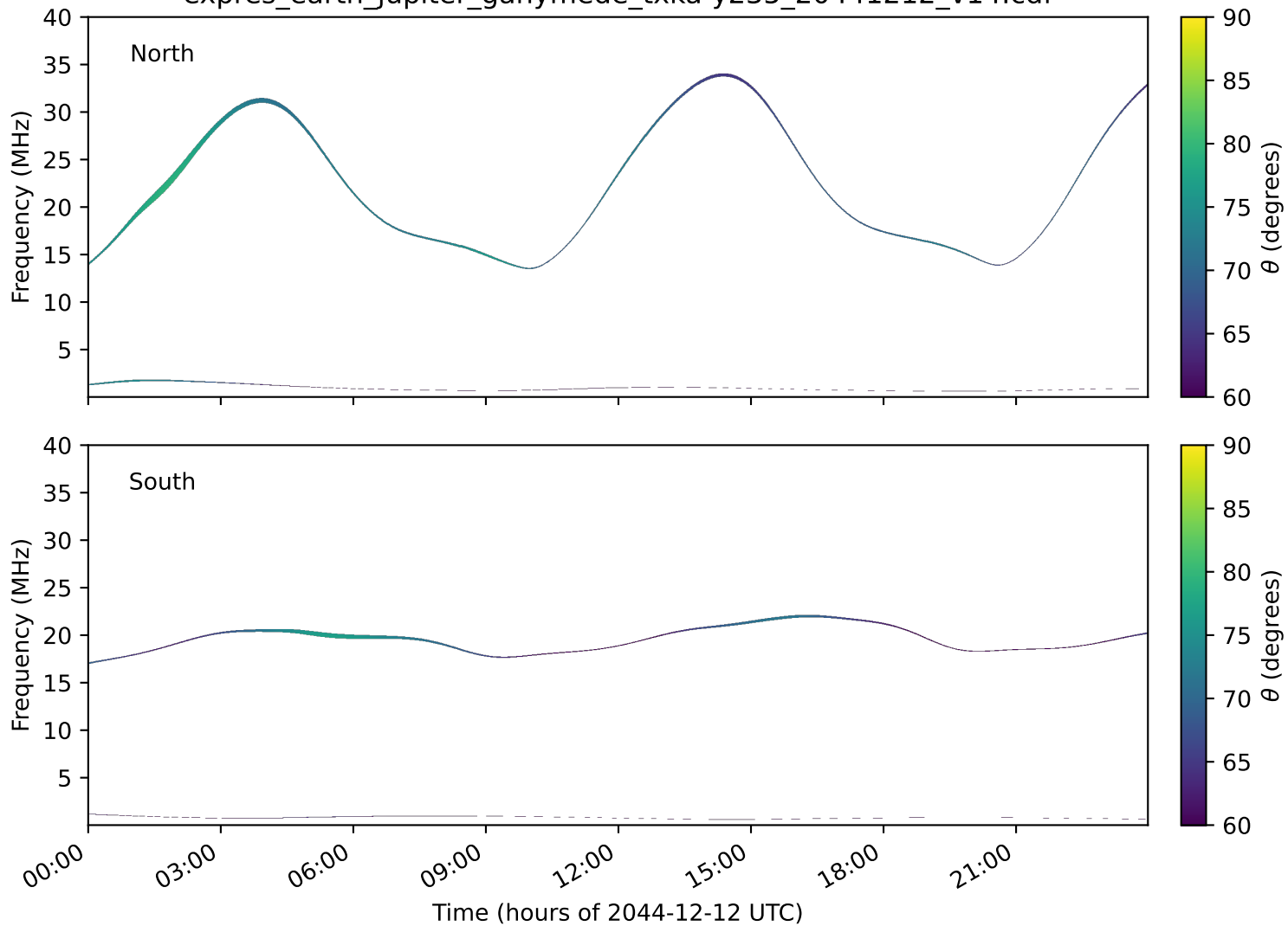
expres_earth_jupiter_ganymede_txka-y235_20441212_v14.cdf
