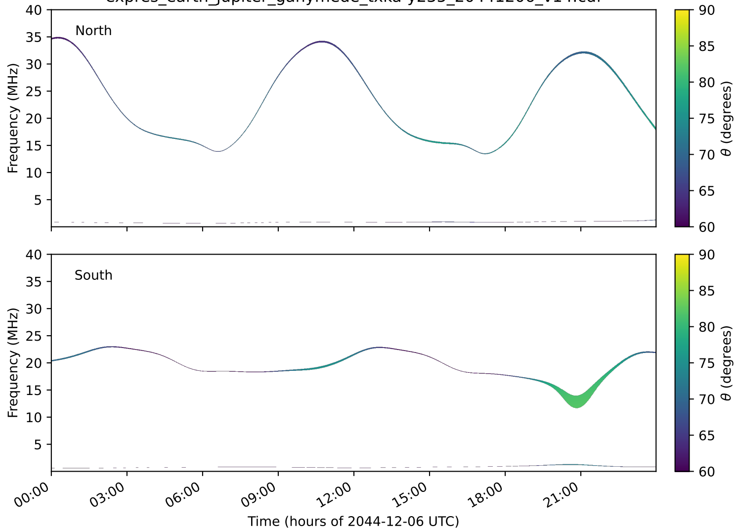
expres_earth_jupiter_ganymede_txka-y235_20441206_v14.cdf
