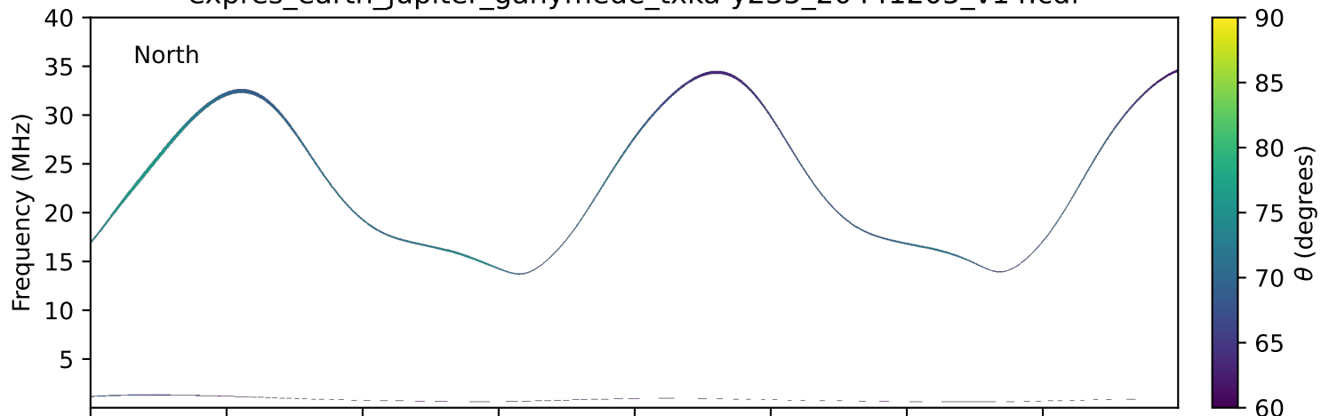
expres_earth_jupiter_ganymede_txka-y235_20441205_v14.cdf
