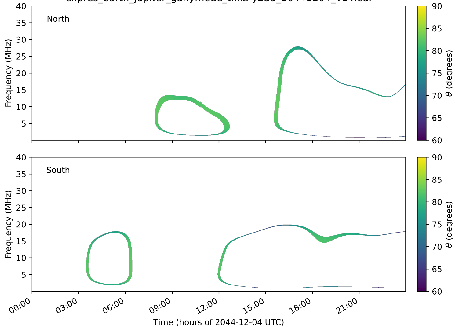
expres_earth_jupiter_ganymede_txka-y235_20441204_v14.cdf
